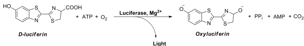
Figure 1. Chemical reaction of luciferin and red firefly luciferase. Light, with an emission maximum of 613nm, is produced from the oxidation of D-luciferin by red firefly luciferase in an ATP-dependent reaction.
