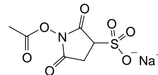
Figure 1. Chemical structure of Sulfo-NHS Acetate.
