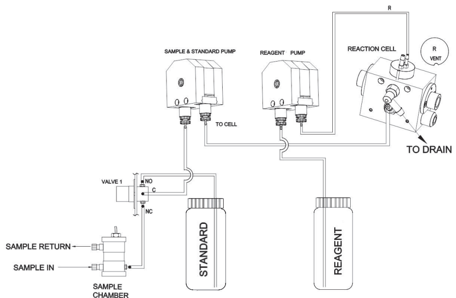
Figure 5: Internal tubing and tube routing interconnections
