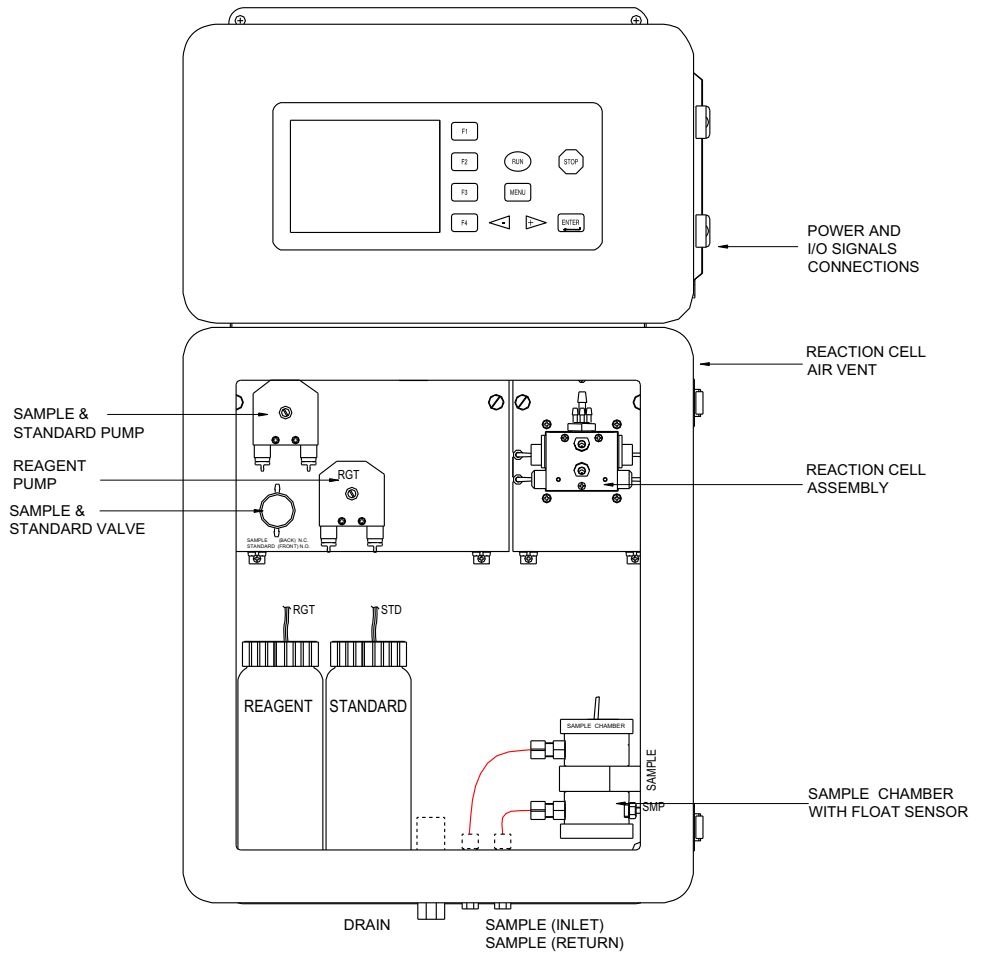
Figure 2: Orion 2295 Phosphate Analyzer PO 4 layout
