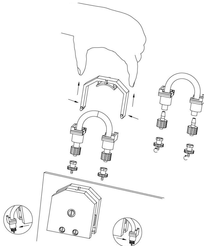
Figure 6: Installing peristaltic pump head tubing - (Single channel)
