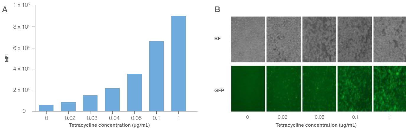
Figure 2: Tetracycline-induced expression of cannabinoid receptor 2 (CB2) in Expi293F Inducible GnTI- cells. Dose response curve shows ability to control expression with Expi293F Inducible GnTI- cells.
