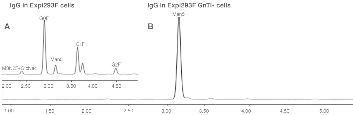
Figure 1: Mass spectrometric analysis of human IgG expressed in Expi293F cells (A) and Expi293F GnTI- cells (B). Expi293F GnTI- cells show uniform glycosylation, with over 98% of glycans expressed being of the Man5 variety.
